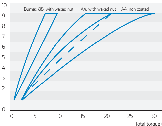
Fig1. Torque/clamp load diagram based on laboratory tests carried out on ISO 4017 bolts, ISO 4032 nuts and ISO 7089 washers of dimension M6.
